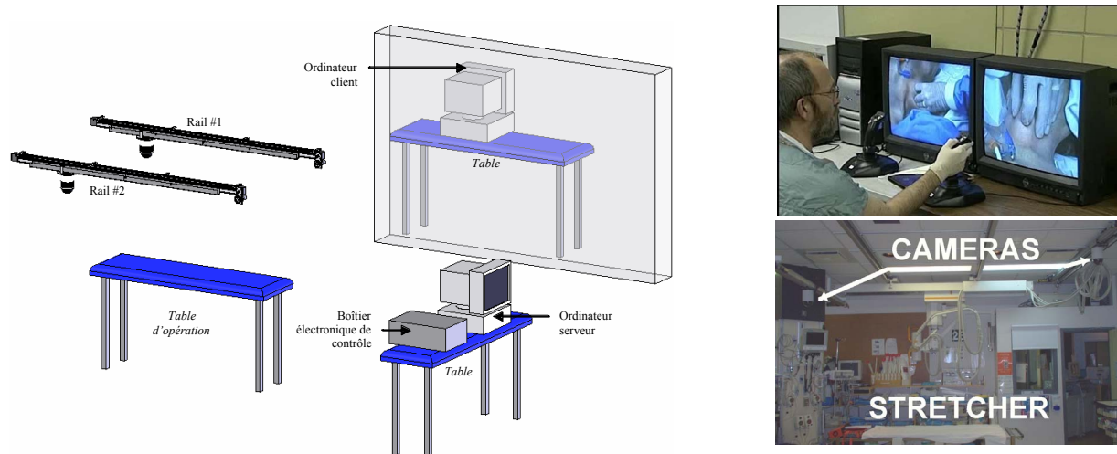
Fig. 1 – Prototype 1 schematics (left), remote control (top right) and installation (bottom right)
